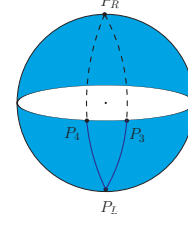
FIG. 2: The path on the Poincaré sphere that determines the geometric phase. The angle \varphi_{34} between the linear polaroids determines the width of the lune on the Poincaré sphere and the geometric phase.
